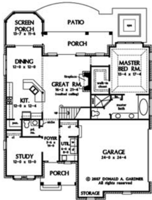
FIRST FLOOR PLAN PLAN NO. 1214
