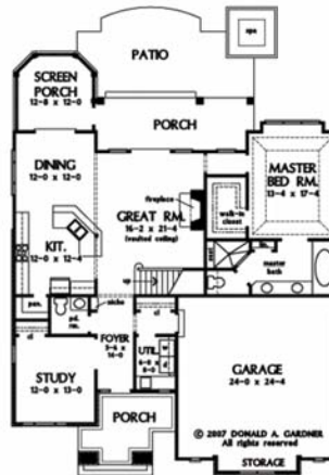
FIRST FLOOR PLAN PLAN NO. 1215
